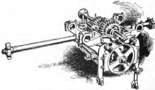
FIG. 379.—Change Speed Gear, used on the heavy gasoline delivery wagons manufactured by the American Daimler Co.
